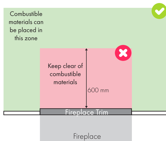
Fig. Top View of the Wall and Fireplace
